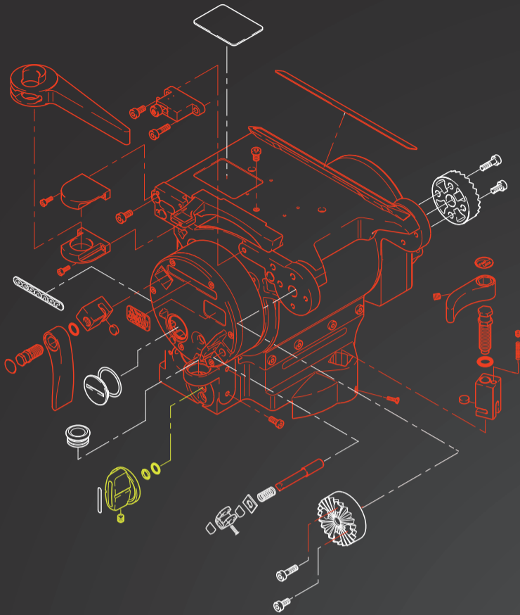
Main Assembly Central Parts
