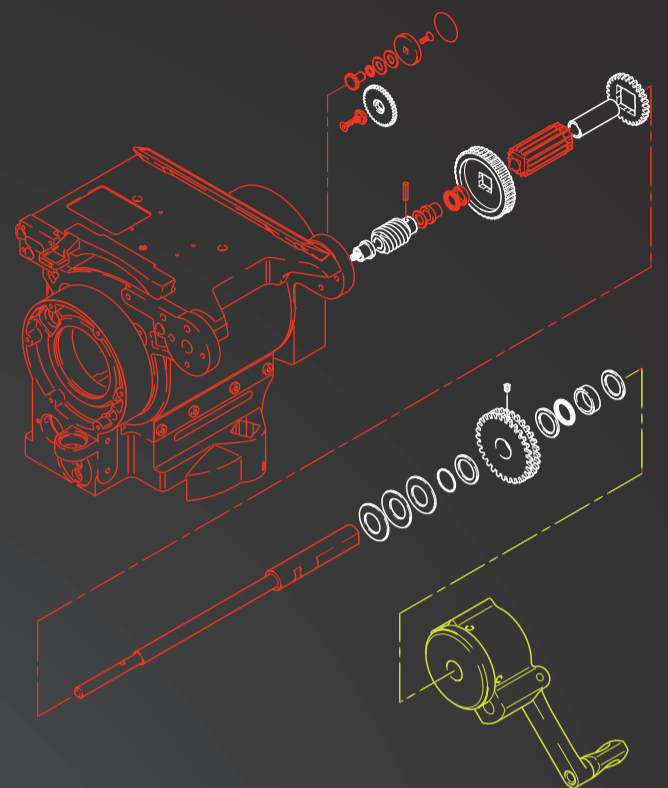
Counter Balance Adjustment
