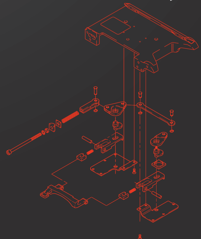
Platform Assembly
