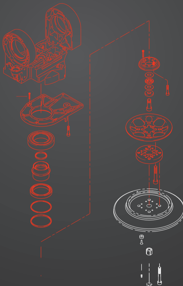
Pan Assembly
