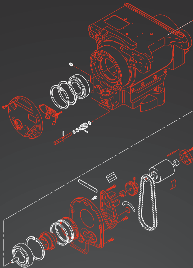
Pan Assembly
