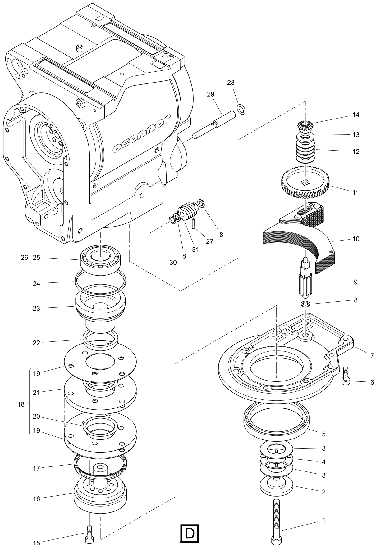
Fig 5.0 Pan Cover End
