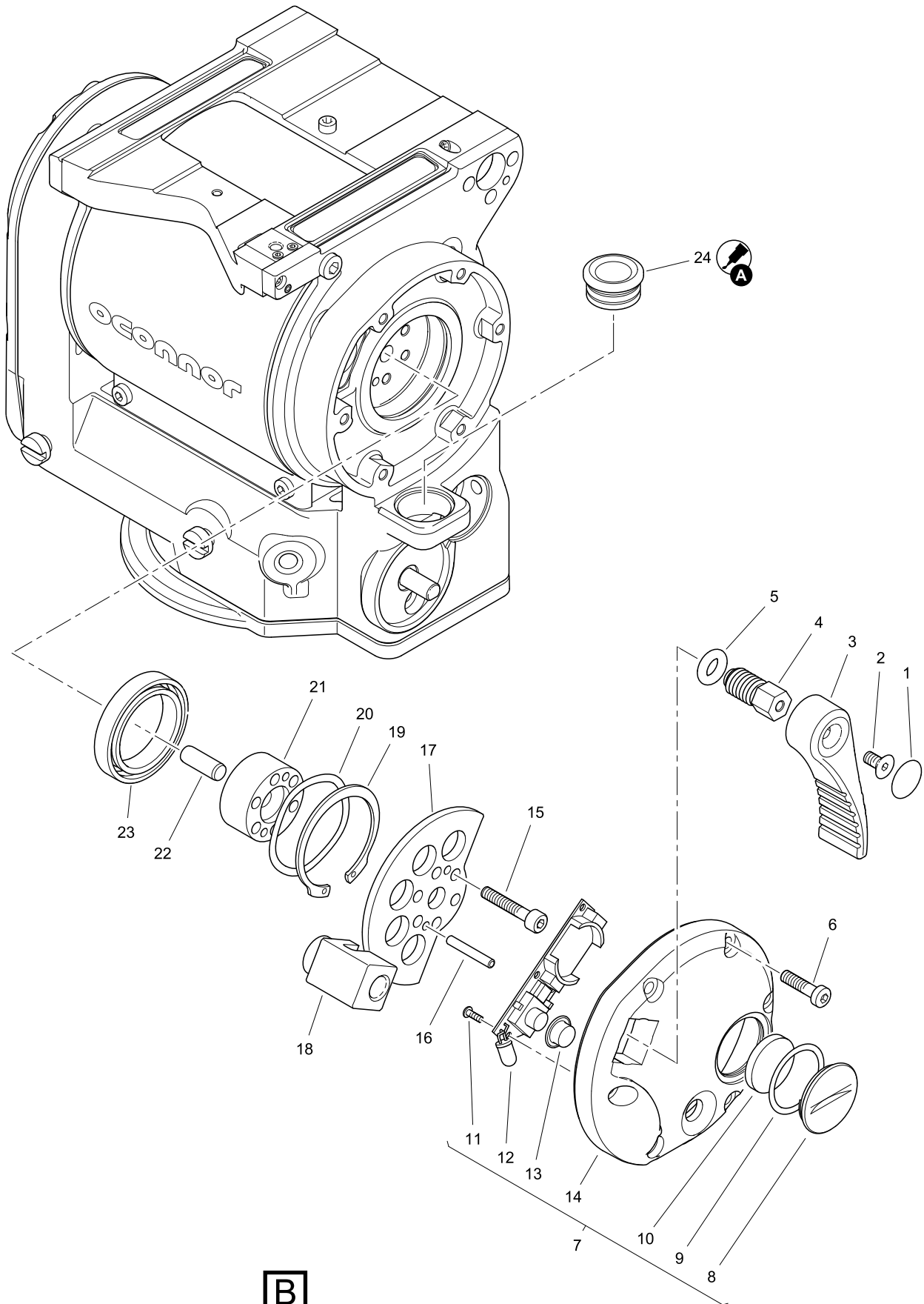
Fig 3.0 Lock Cover End
