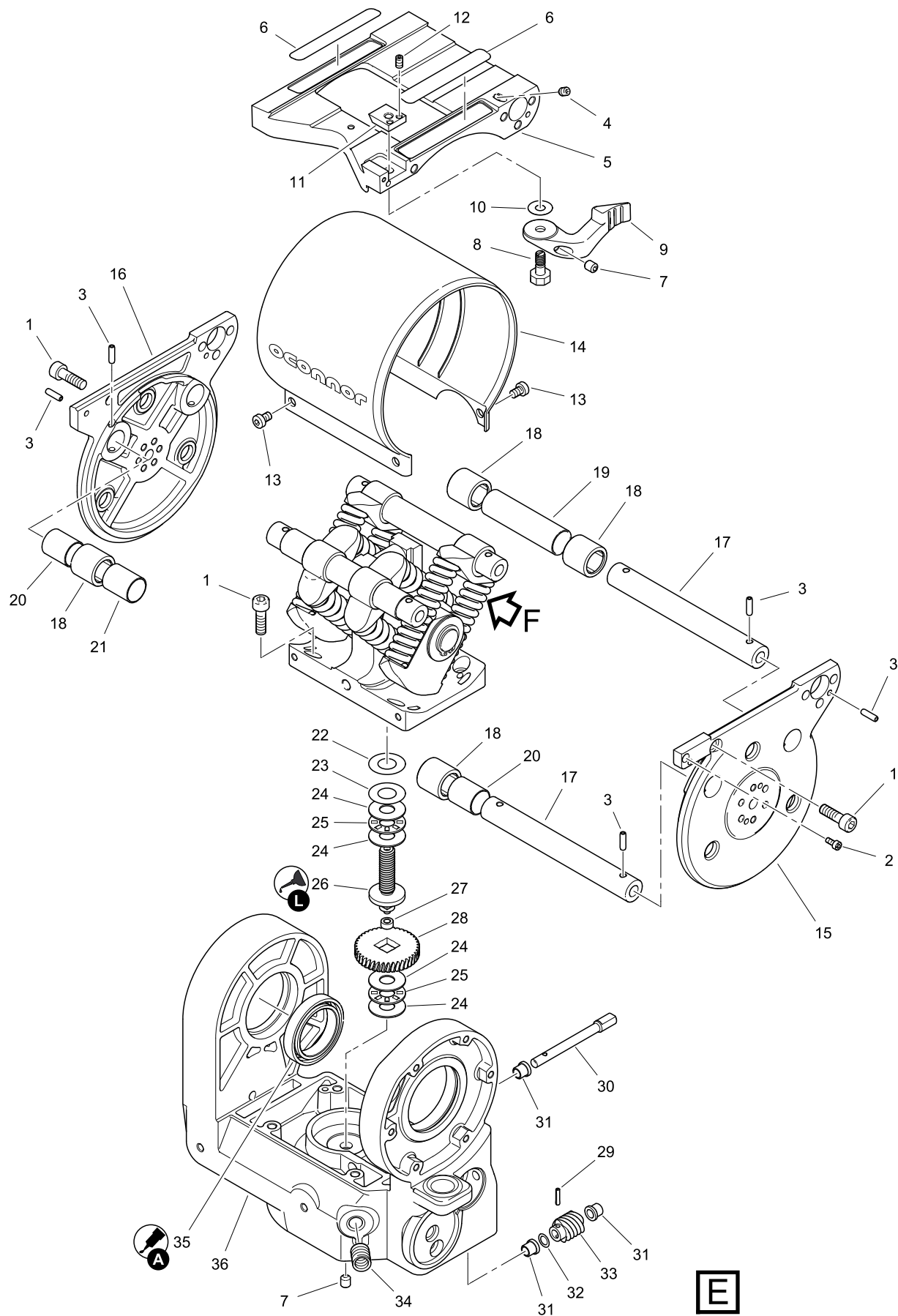
Fig 6.0 Main Body
