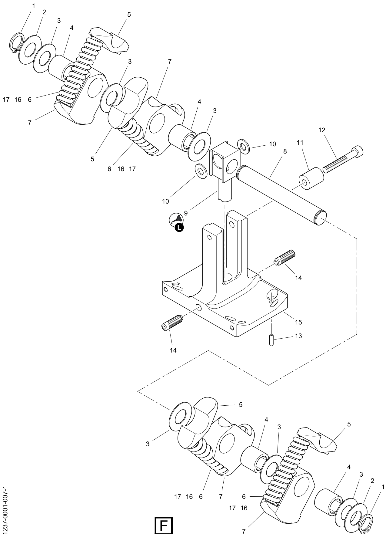
Fig 7.0 Counter Balance Adjustment
