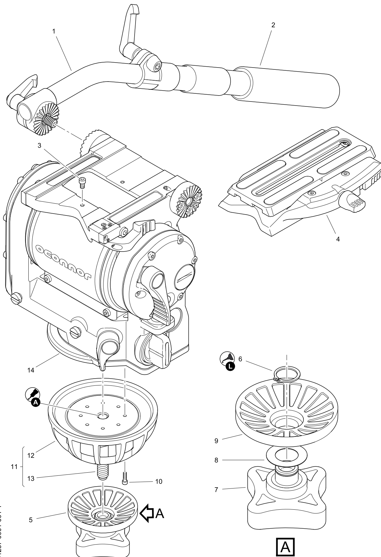
Fig 1.0 1030D Configured Assembly
