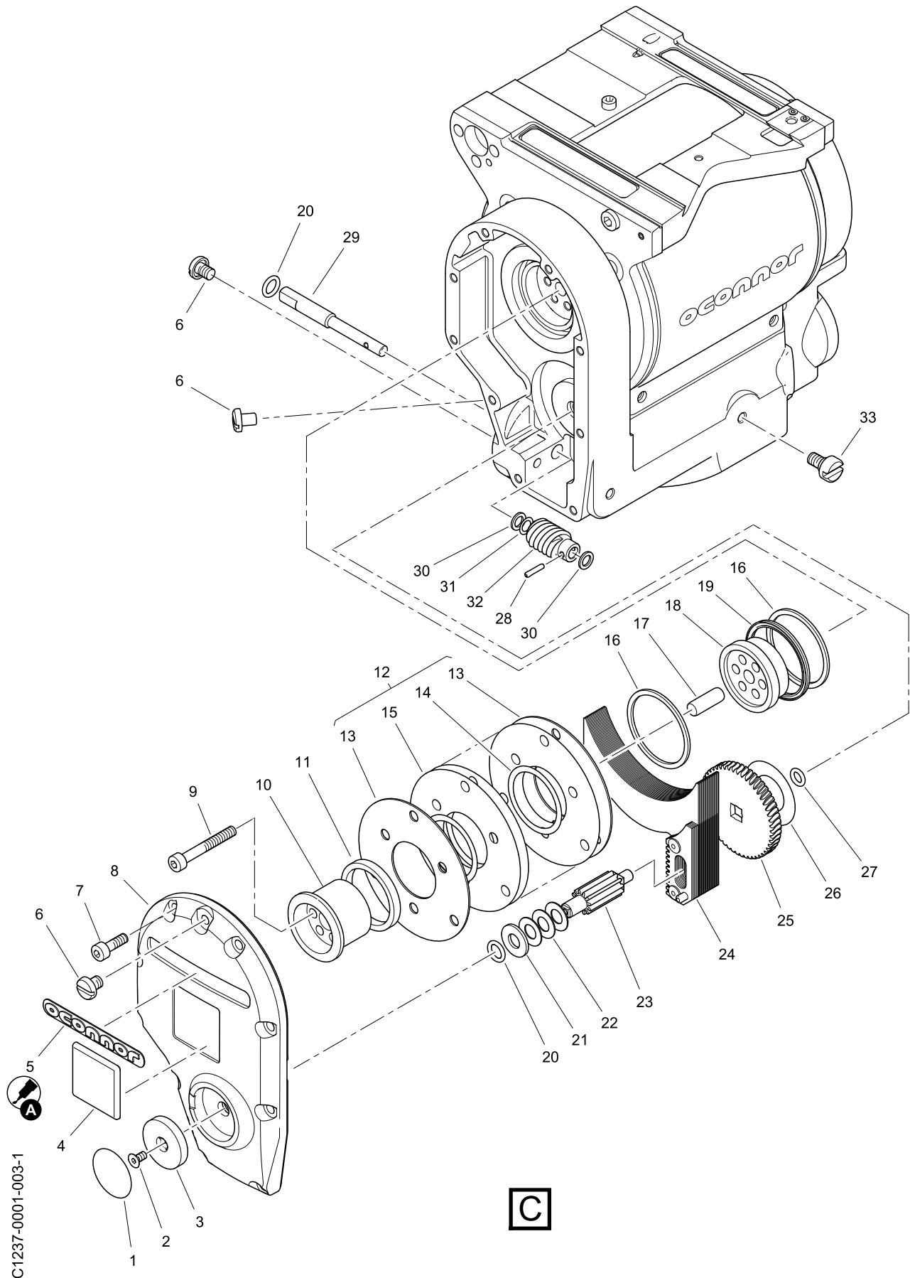
Fig 4.0 Fluid Cover End
